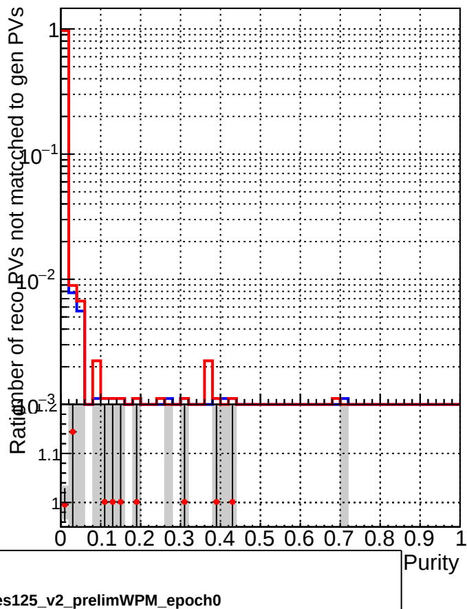
RecoPVAssoc2GenPVNotMatched_missing
