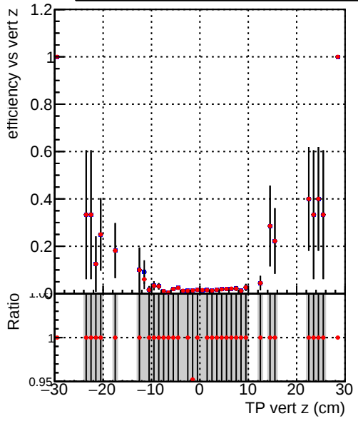
Efficiency vs. TP vert z (cm) —●— DQM_CKF_XiMinusPU_base —●— DQM_CKF_XiMinusPU_retrainOldFiles125_v2_prelimWPM_epoch0
