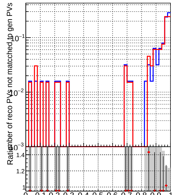
RecoPVAssoc2GenPVNotMatched_missing
