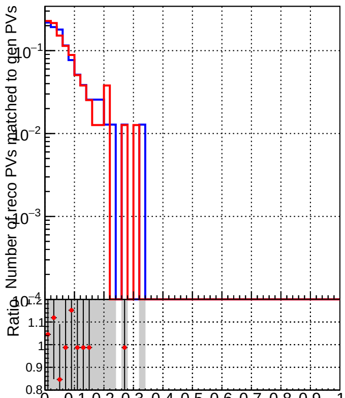
RecoPVAssoc2GenPVMatched_missing
