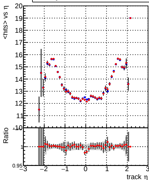
mean hits vs \eta Legend: DQM_CKF_XiMinusPU_base (blue line), DQM_CKF_XiMinusPU_retrainOldFiles125_v2_prelimWPM_epoch0 (red line)
