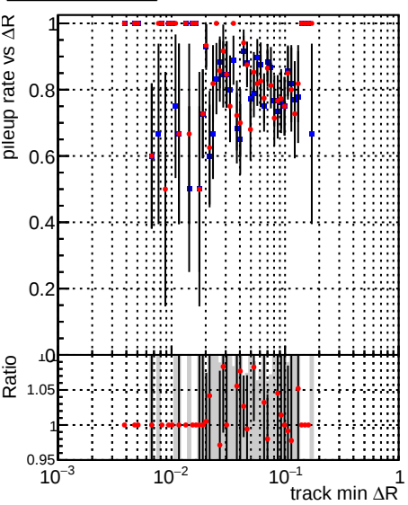
Legend: DQM_CKF_XiMinusPU_base (blue squares), DQM_CKF_XiMinusPU_retrainOldFiles125_v2_prelimWPM_epoch0 (red circles)
