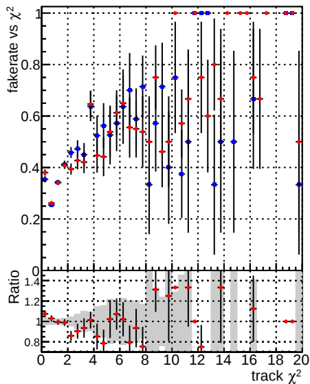
Fake rate vs. \chi^2 —●— DQM_CKF_XiMinusPU_base —●— DQM_CKF_XiMinusPU_retrainOldFiles125_v2_prelimWPM_epoch0
