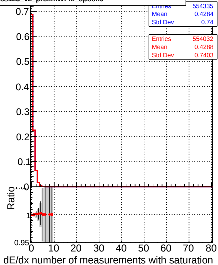
Legend: \blacksquare DQM_CKF_XiMinusPU_base \bullet DQM_CKF_XiMinusPU_retrainOldFiles125_v2_prelimWPM_epoch0
