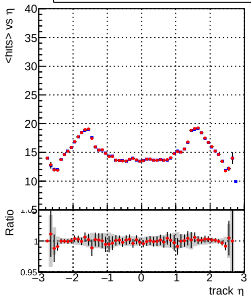
mean hits vs \eta — DQM_CKF_XiMinusPU_base — DQM_CKF_XiMinusPU_retrainOldFiles125_v2_prelimWPM_epoch0
