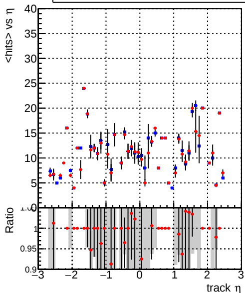
mean hits vs \eta Legend: DQM_CKF_XiMinusPU_base (blue line with dots), DQM_CKF_XiMinusPU_retrainOldFiles125_v2_prelimWPM_epoch0 (red line with dots)
