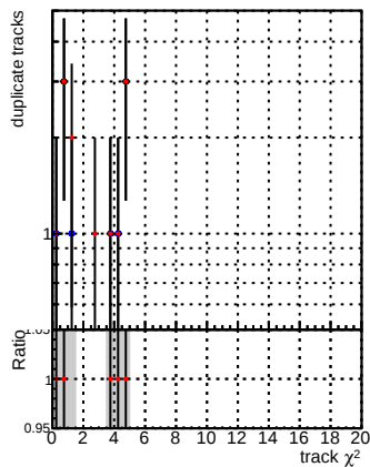
N of associated (recoToSim) loopor tracks vs normalized \chi^2
