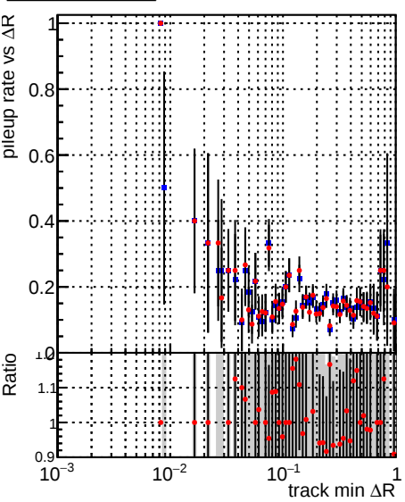
Legend: DQM_CKF_XiMinusPU_base (blue), DQM_CKF_XiMinusPU_retrainOldFiles125_v2_prelimWPM_epoch0 (red)
