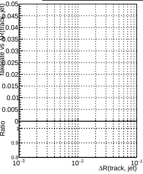
Legend: DQM_CKF_XiMinusPU_base (blue), DQM_CKF_XiMinusPU_retrainOldFiles125_v2_prelimWPM_epoch0 (red)
