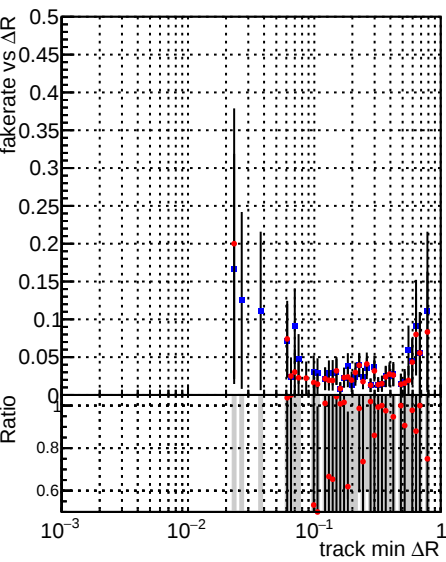
Legend: DQM_CKF_XiMinusPU_base (blue), DQM_CKF_XiMinusPU_retrainOldFiles125_v2_prelimWPM_epoch0 (red)
