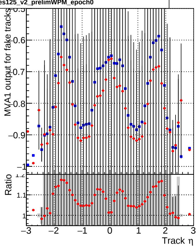
MVA1 of non-associated tracks (recoToSim) vs. track \eta
