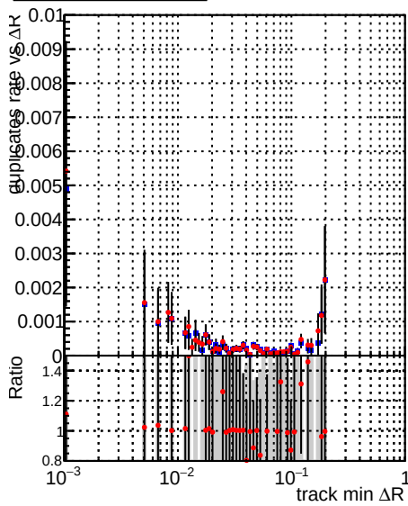
Legend: DQM_CKF_XiMinusPU_base (blue points), DQM_CKF_XiMinusPU_retrainOldFiles125_v2_prelimWPM_epoch0 (red points)
