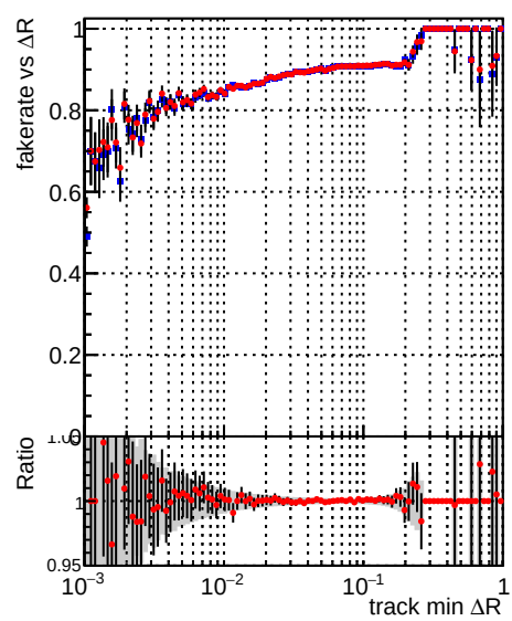
Legend: DQM_CKF_XiMinusPU_base (blue points), DQM_CKF_XiMinusPU_retrainOldFiles125_v2_prelimWPM_epoch0 (red points)
