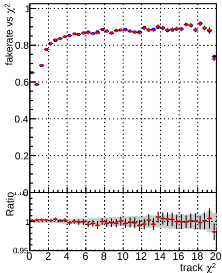
Fake rate vs. \chi^2 Legend: DQM_CKF_XiMinusPU_base (blue stars) DQM_CKF_XiMinusPU_retrainOldFiles125_v2_prelimWPM_epoch0 (red stars)
