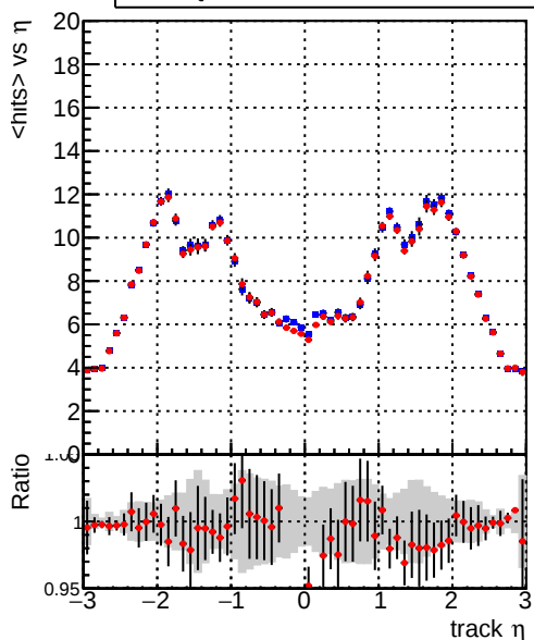
mean hit — DQM_CKF_XiMinusPU_base — DQM_CKF_XiMinusPU_retrainOldFiles125_v2_prelimWPM_epoch0
