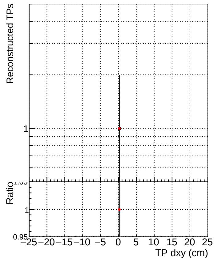
Legend: ■ DQM_CKF_XiMinusPU_base ● DQM_CKF_XiMinusPU_retrainOldFiles125_v2_prelimWPM_epoch0
