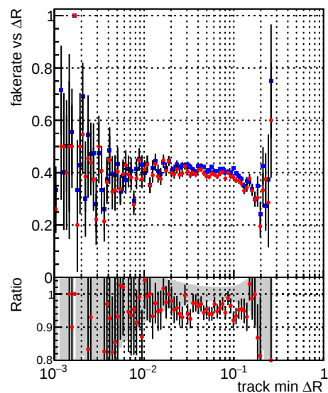
Fake rate vs \Delta R(\text{track, jet}) DQM_CKF_XiMinusPU_base DQM_CKF_XiMinusPU_retrainOldFiles125_v2_prelimWPM_epoch0
