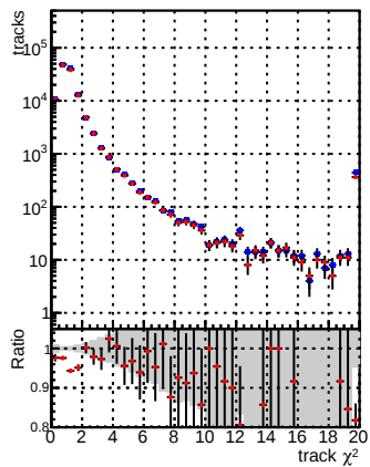
N of reco track vs. DQM_CKF_XiMinusPU_base DQM_CKF_XiMinusPU_retrainOldFiles125_v2_prelimWPM_epoch0
