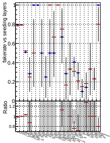
Fake rate vs. Legend: DQM CKF XiMinusPU base (blue) DQM CKF XiMinusPU retrainOldFiles125 v2_prelimWPM_epoch0 (red)
