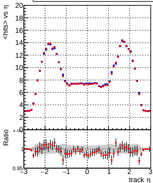
mean hits vs \eta — DQM_CKF_XiMinusPU_base — DQM_CKF_XiMinusPU_retrainOldFiles125_v2_prelimWPM_epoch0
