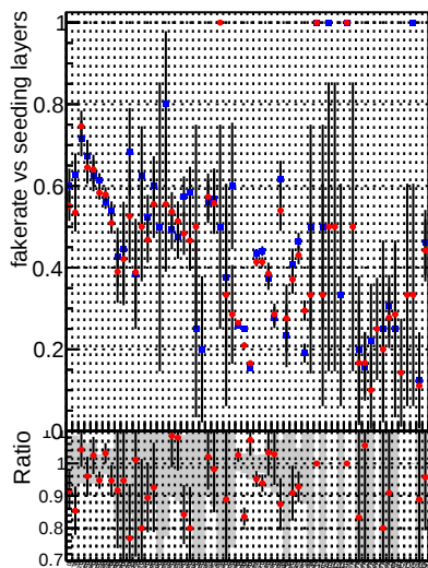
Fake rate vs. —◆— DQM CKF_XiMinusPU_base —★— DQM CKF_XiMinusPU_retrainOldFiles125_v2_prelimWPM_epoch0
