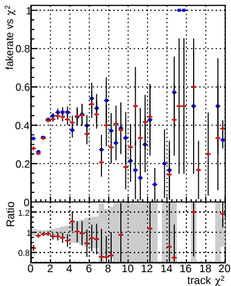
Fake rate vs. —◆— DQM CKF_XiMinusPU_base —★— DQM CKF_XiMinusPU_retrainOldFiles125_v2_prelimWPM_epoch0
