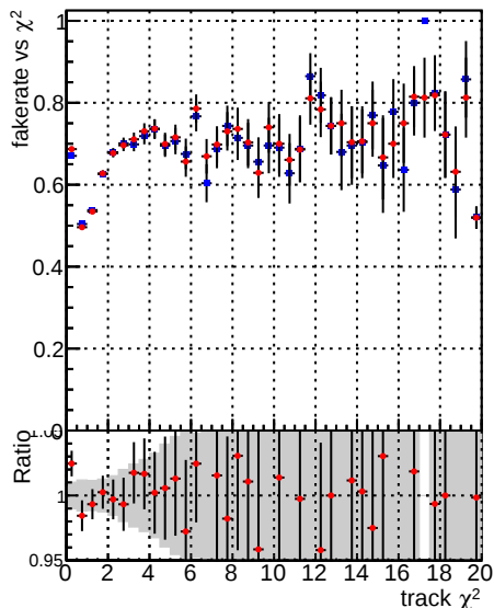
Fake rate vs. \chi^2 Legend: —●— DQM_CKF_XiMinusPU_base —●— DQM_CKF_XiMinusPU_retrainOldFiles125_v2_prelimWPM_epoch0
