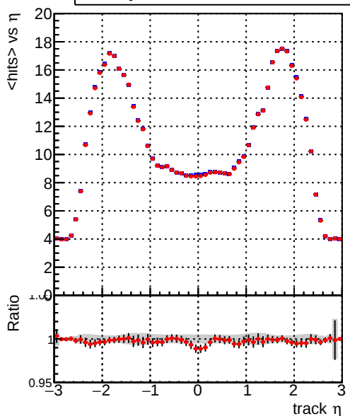
mean hit — DQM_CKF_XiMinusPU_base — DQM_CKF_XiMinusPU_retrainOldFiles125_v2_prelimWPM_epoch0
