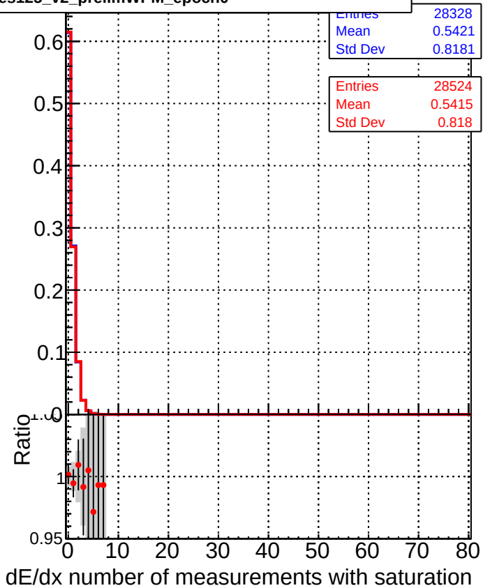
—■— DQM_CKF_XiMinusPU_base —●— DQM_CKF_XiMinusPU_retrainOldFiles125_v2_prelimWPM_epoch0
