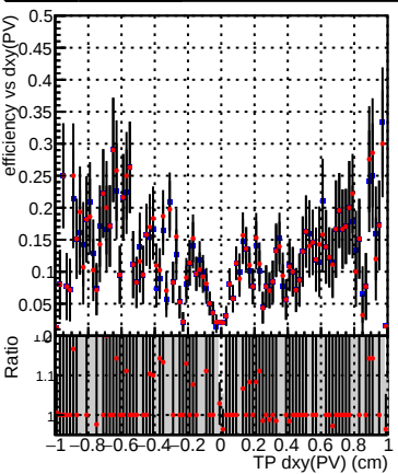
Efficiency vs Dxy(PV) Legend: DQM_CKF_XiMinusNOPU_base (blue squares), DQM_CKF_XiMinusNOPU_retrainOldFiles125_v2_prelimWPM_epoch4 (red circles)
