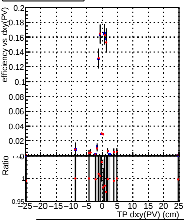
Efficiency vs Dxy(PV) Legend: DQM_CKF_XiMinusNOPU_base (blue squares), DQM_CKF_XiMinusNOPU_retrainOldFiles125_v2_prelimWPM_epoch4 (red circles)
