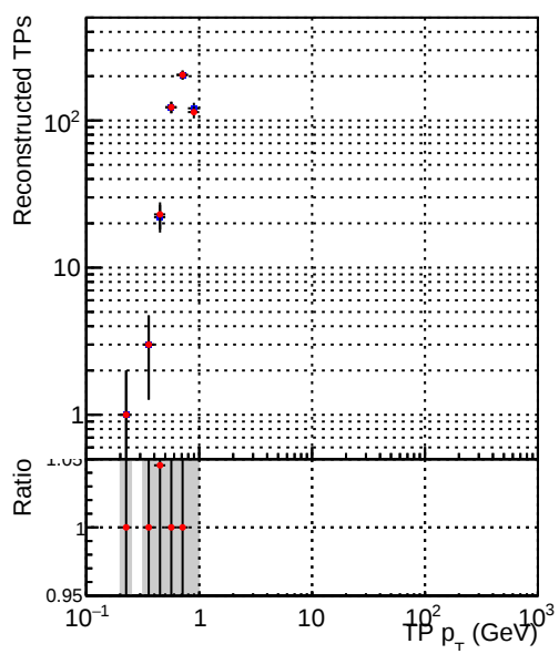
Legend: \blacksquare DQM_CKF_XiMinusNOPU_base \blacklozenge DQM_CKF_XiMinusNOPU_retrainOldFiles125_v2_prelimWPM_epoch4
