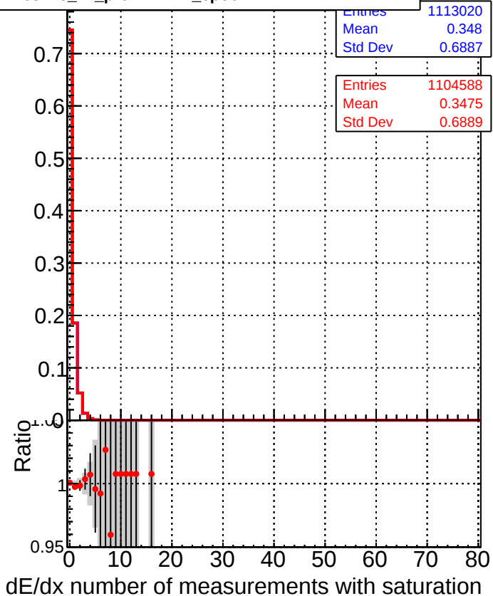
Legend: DQM_CKF_XiMinusNOPU_base (blue line with squares), DQM_CKF_XiMinusNOPU_retrainOldFiles125_v2_prelimWPM_epoch4 (red line with circles)
