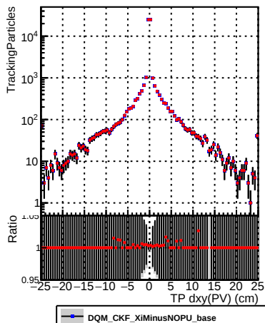
N of sim —●— DQM_CKF_XiMinusNOPU_retrainOldFiles125_v2_prelimWPM_epoch4
