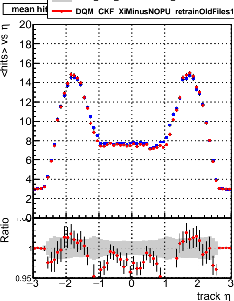
mean hits
