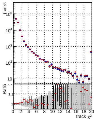
N of reco track vs. \chi^2 —•— DQM_CKF_XiMinusNOPU_base —•— DQM_CKF_XiMinusNOPU_retrainOldFiles125_v2_prelimWPM_epoch4
