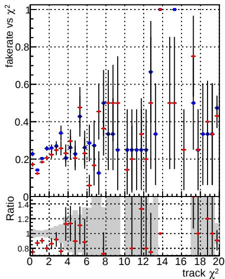
Fake rate vs. \chi^2 ◆ DQM_CKF_XiMinusNOPU_base ★ DQM_CKF_XiMinusNOPU_retrainOldFiles125_v2_prelimWPM_epoch4
