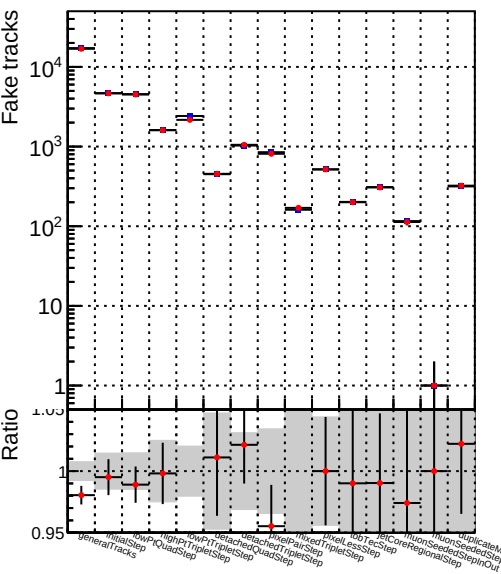
Number 1 DQM_CKF_XiMinusNOPU_retrainOldFiles125_v2_prelimWPM_epoch4
