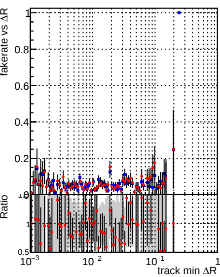
Legend: DQM_CKF_XiMinusNOPU_base (blue stars), DQM_CKF_XiMinusNOPU_retrainOldFiles125_v2_prelimWPM_epoch4 (red stars)
