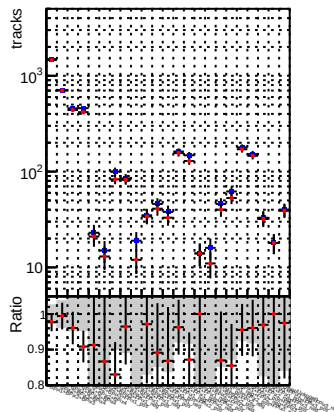
N of reco track vs. \chi^2 for DOM CKF XiMinusNOPU_base and DOM CKF XiMinusNOPU_retrainOldFiles125_v2_prelimWPM_epoch4 models.
