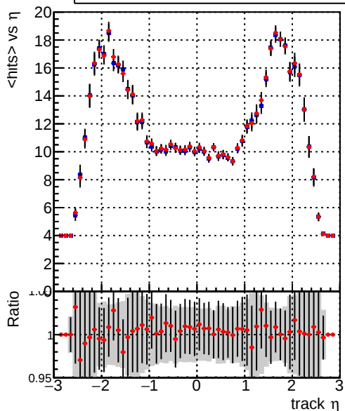
mean hit — DQM_CKF_XiMinusNOPU_base — DQM_CKF_XiMinusNOPU_retrainOldFiles125_v2_prelimWPM_epoch4
