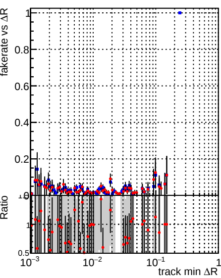
Fake rate vs \Delta R(\text{track, jet}) DQM_CKF_XiMinusNOPU_base DQM_CKF_XiMinusNOPU_retrainOldFiles125_v2_prelimWPM_epoch4
