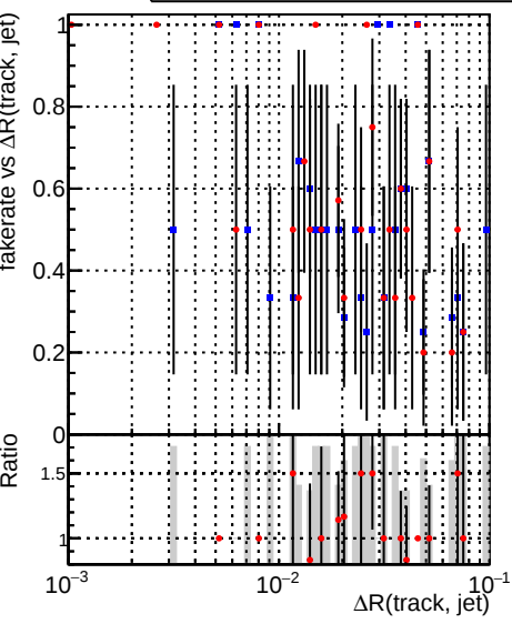
Fake rate vs \Delta R(\text{track, jet}) Legend: —•— DQM_CKF_XiMinusNOPU_base —•— DQM_CKF_XiMinusNOPU_retrainOldFiles125_v2_prelimWPM_epoch4
