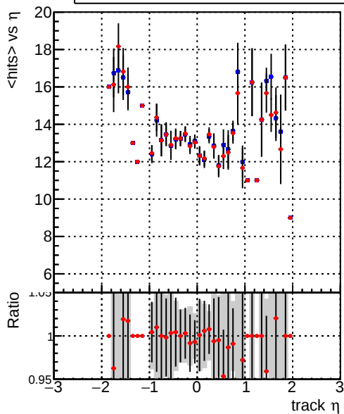
mean hit — DQM_CKF_XiMinusNOPU_base — DQM_CKF_XiMinusNOPU_retrainOldFiles125_v2_prelimWPM_epoch4
