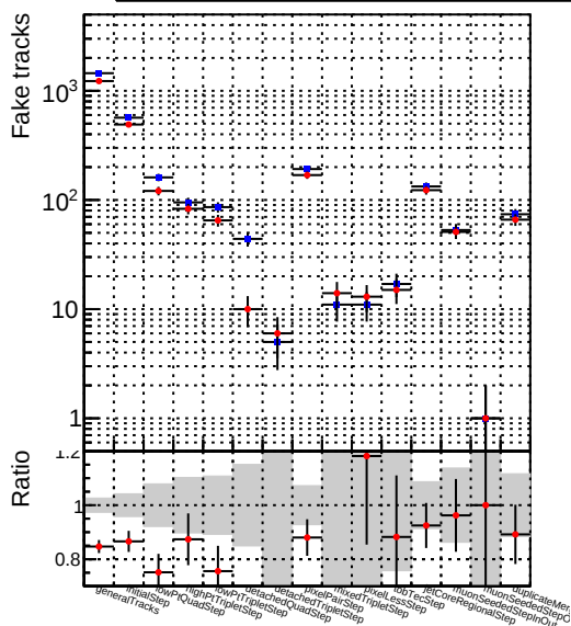
DOM CKE XiMinusNOPU retrainOldFiles125 v2 prelimWPM epoch4 Number —● —● —● —● —● —●
