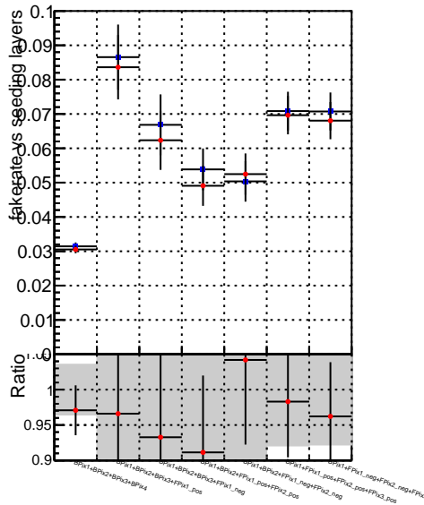
Fake rate vs. —•— DQM_CKF_XiMinusNOPU_base —•— DQM_CKF_XiMinusNOPU_retrainOldFiles125_v2_prelimWPM_epoch4
