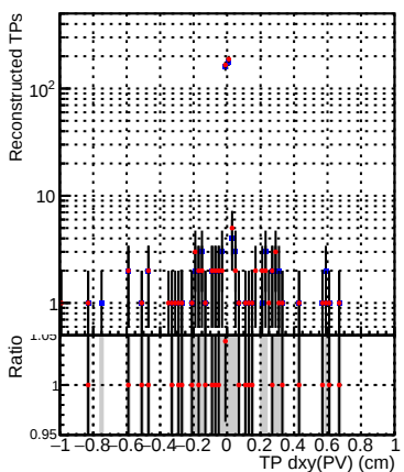
N of sim DQM_CKF_XiMinusNOPU_retrainOldFiles125_v2_prelimWPM_epoch4
