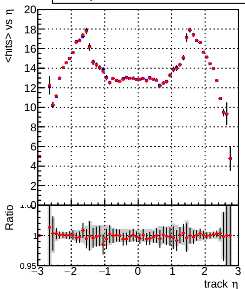
mean hits vs \eta — DQM_CKF_XiMinusNOPU_base — DQM_CKF_XiMinusNOPU_retrainOldFiles125_v2_prelimWPM_epoch4
