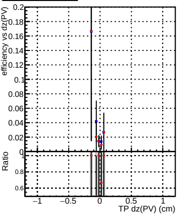
Efficiency vs Dz(PV) plot
