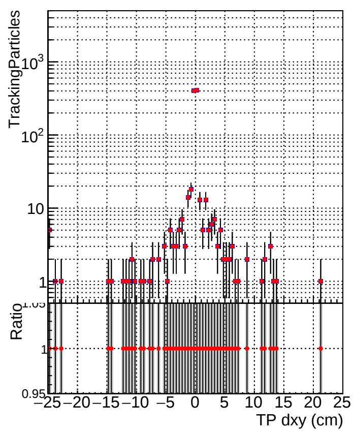
N of simulated track DQM_CKF_XiMinusNOPU_base DQM_CKF_XiMinusNOPU_retrainOldFiles125_v2_prelimWPM_epoch4
