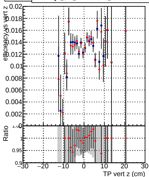
Efficiency — DQM_CKF_XiMinusNOPU_retrainOldFiles125_v2_prelimWPM_epoch4
