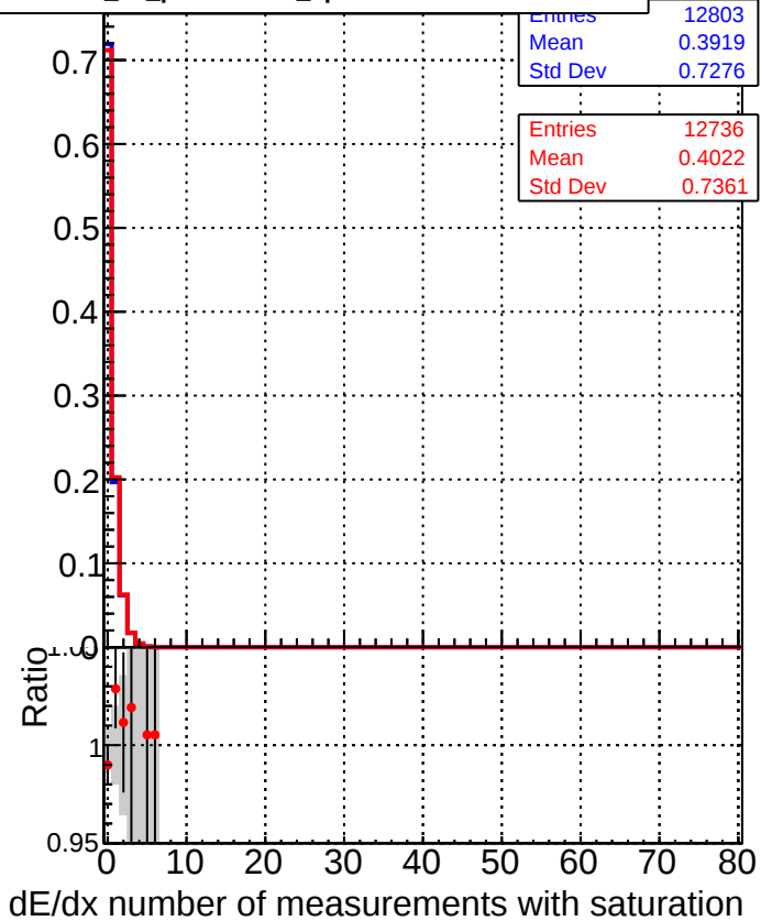
Legend: DQM_CKF_XiMinusNOPU_base (Blue line with square markers) DQM_CKF_XiMinusNOPU_retrainOldFiles125_v2_prelimWPM_epoch4 (Red line with circle markers)
