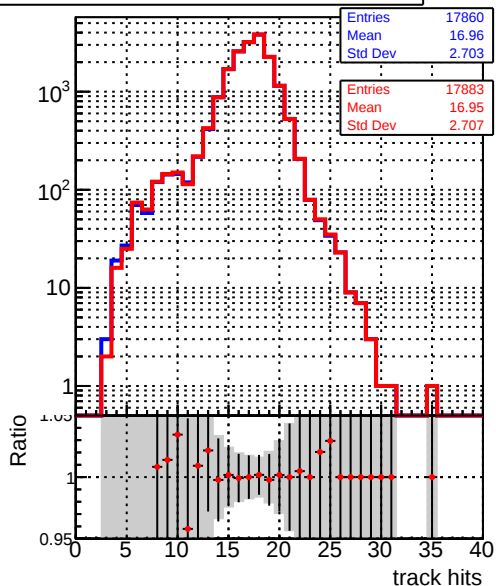
mean hit — DQM_CKF_XiMinusNOPU_base — DQM_CKF_XiMinusNOPU_retrainOldFiles125_v2_prelimWPM_epoch4
