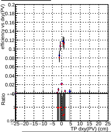
Efficiency vs Dxy(PV) Legend: DQM_CKF_XiMinusNOPU_base (black line with blue markers), DQM_CKF_XiMinusNOPU_retrainOldFiles125_v2_prelimWPM_epoch3 (red line with red markers)
