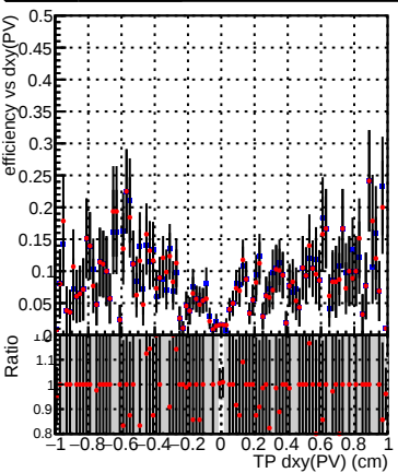
Efficiency vs Dxy(PV) Legend: DQM_CKF_XiMinusNOPU_base (black line with blue markers), DQM_CKF_XiMinusNOPU_retrainOldFiles125_v2_prelimWPM_epoch3 (red line with red markers)
