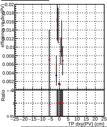
Efficiency vs Dxy(PV) plot
