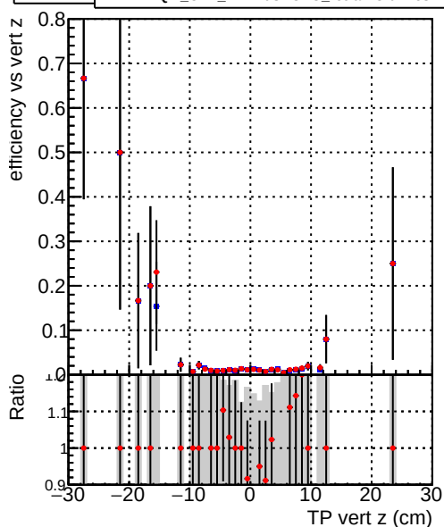
Efficiency vs. sim PV z —●— DQM_CKF_XiMinusNOPU_base —●— DQM_CKF_XiMinusNOPU_retrainOldFiles125_v2_prelimWPM_epoch3
